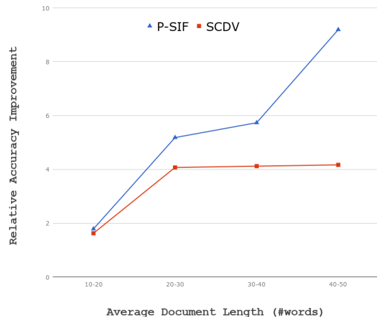
Relative Performance vs Document Length
