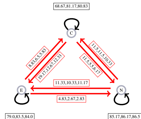
Figure 4: Consistency graph for predictions of ADAPET(token) vs (a) RoBERTa L +CLS (b) ADAPET (pretrained mixNLI) (c) ADAPET (pre-trained MNL) in that order respectively.
